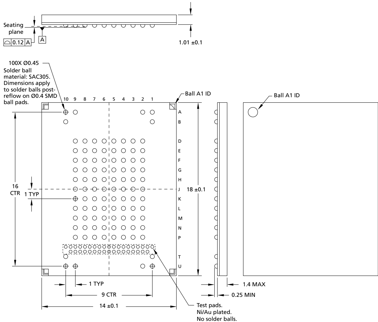
Figure 4: 100-Ball LBGGA – 14.0mm x 18.00mm x 1.4mm (Package Code 1A3)
