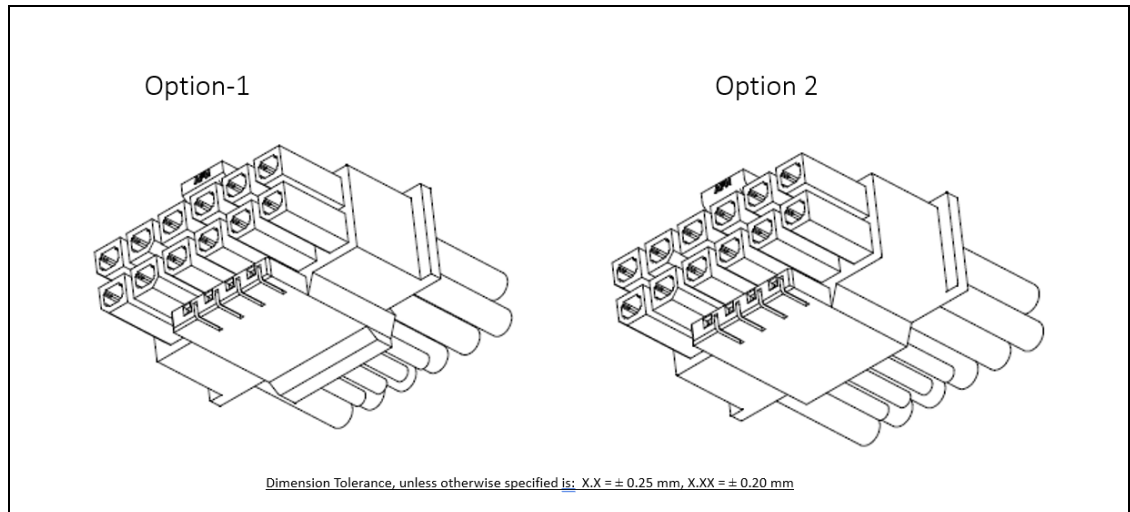
Figure 5-3. 12VHPWR Cable Plug Connector
