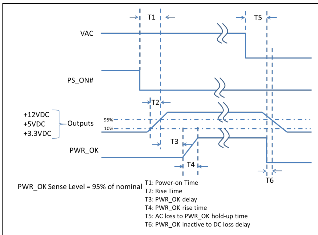
Figure 4-3. Power on Timing
