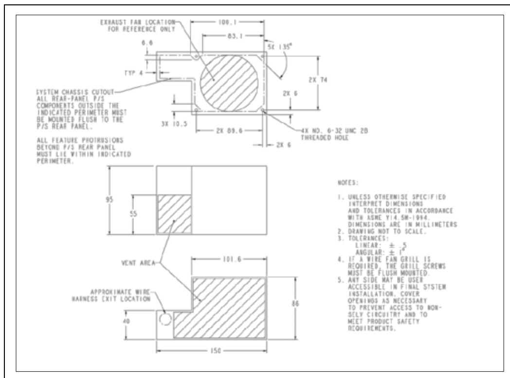
Figure 11-1. CFX12V Mechanical Outline
