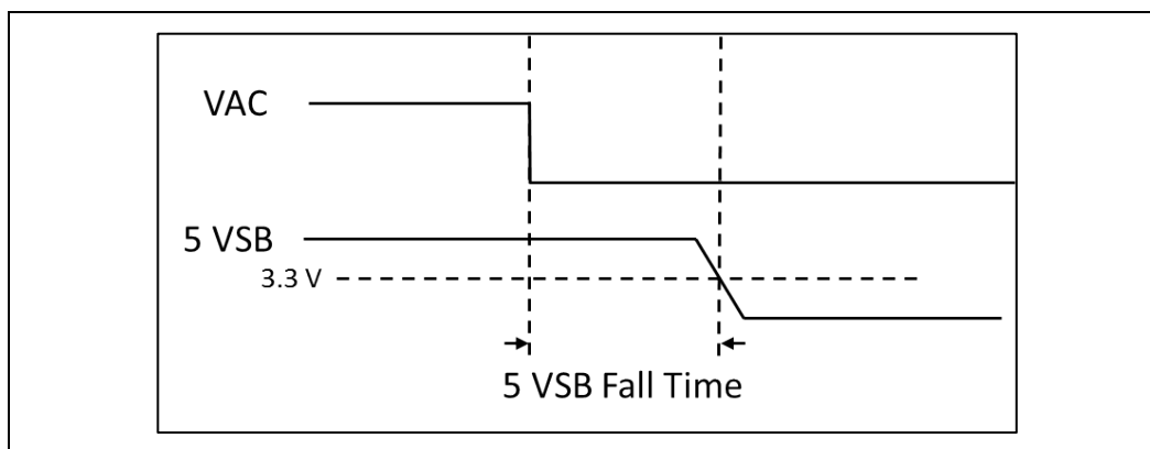
Figure 4-7. 5VSB Fall Time
