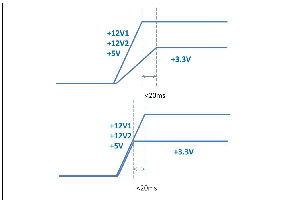
Figure 4-2. Power Supply Timing
