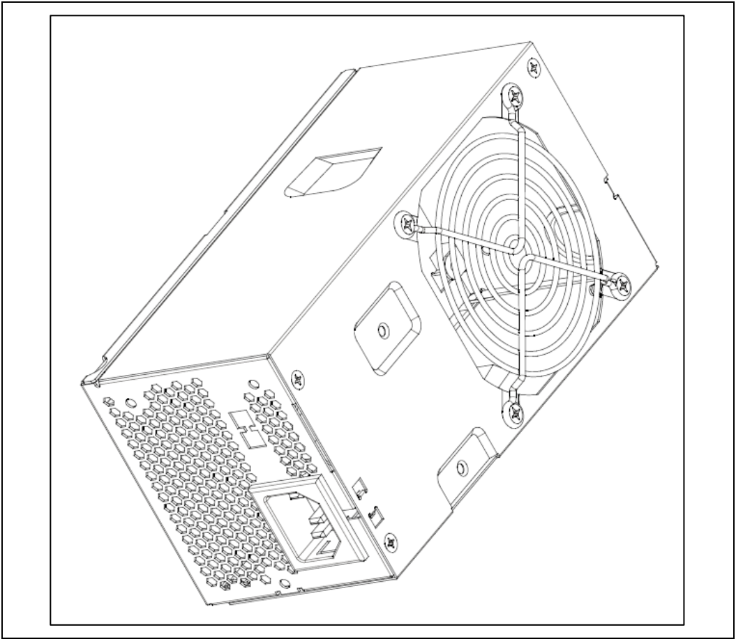
Figure 15-1. Mechanical Outline
