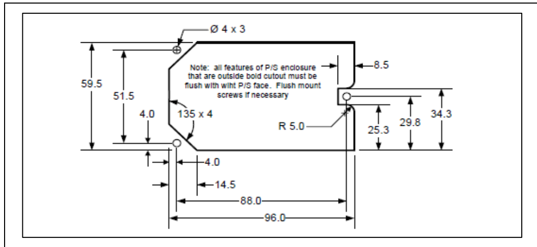
Figure 14-9. Chassis Cutout
