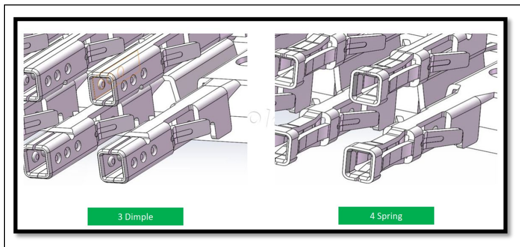
Figure 5-5. 12VHPWR Cable Plug Connection Recommendation
