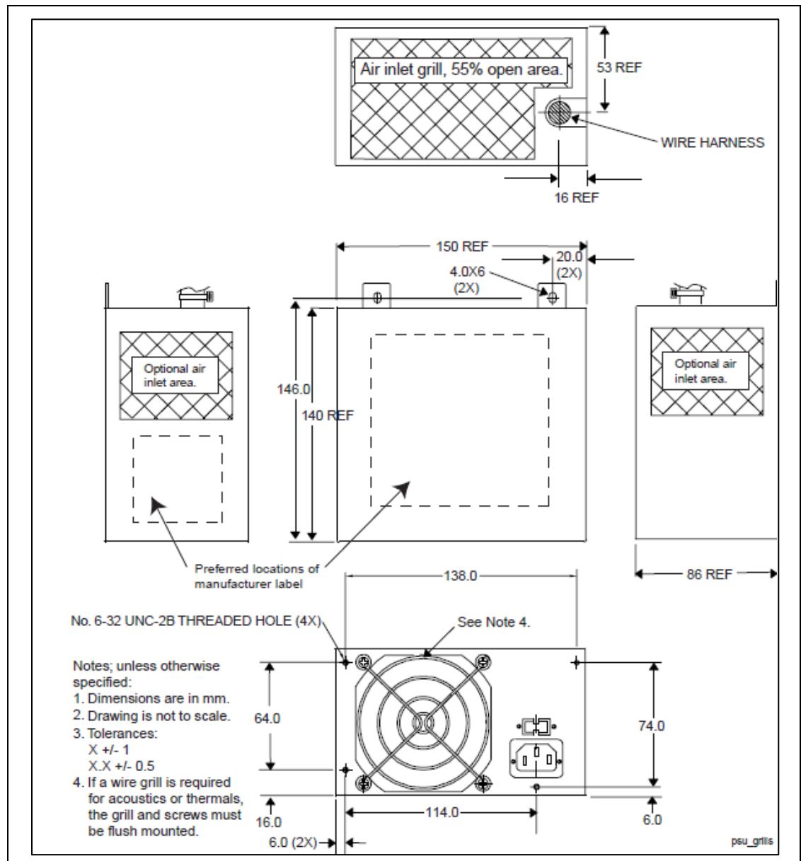
Figure 13-1. Power Supply Dimensions for Chassis that does not Require Top Venting
