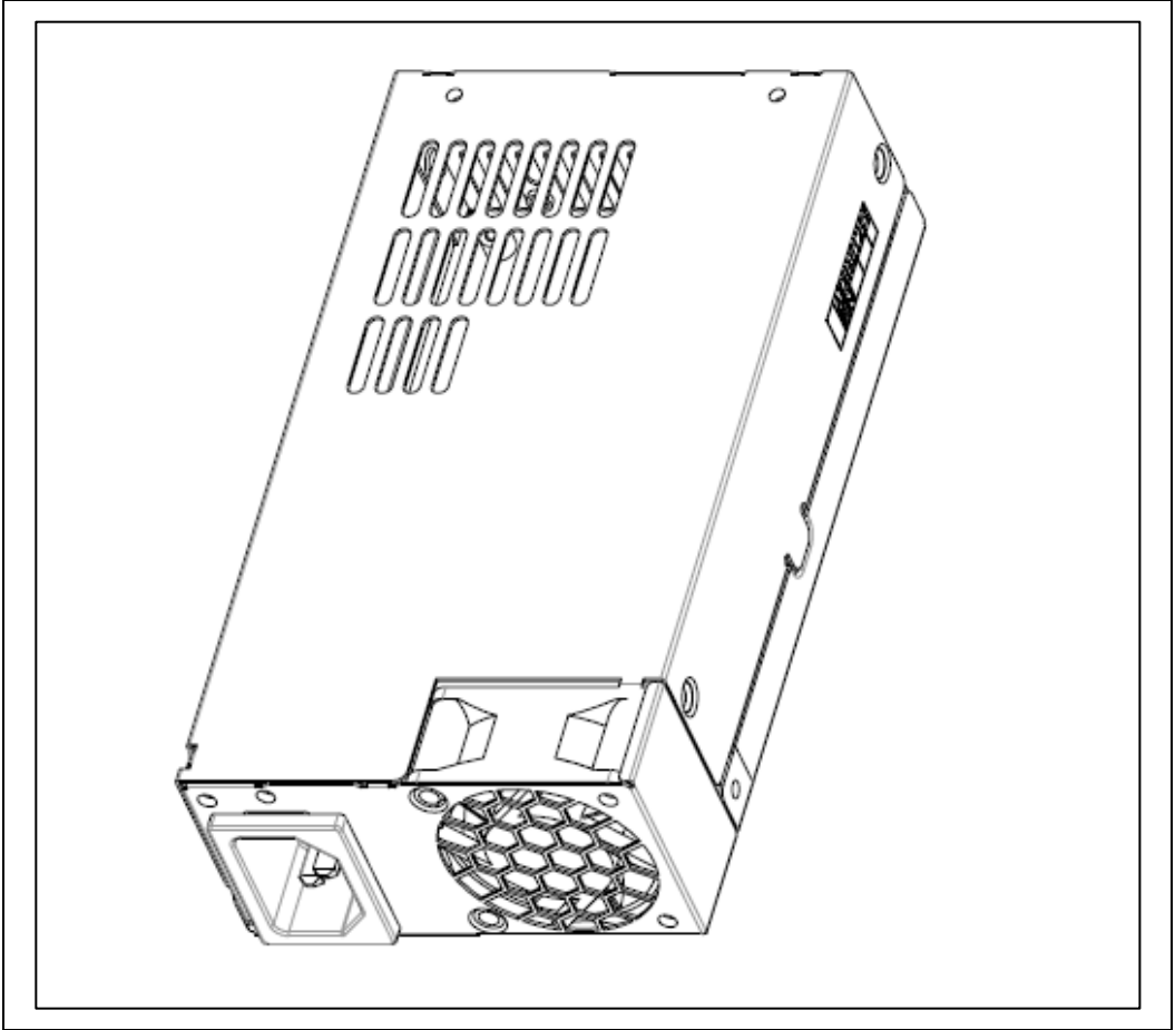
Figure 16-1. Mechanical Outline
