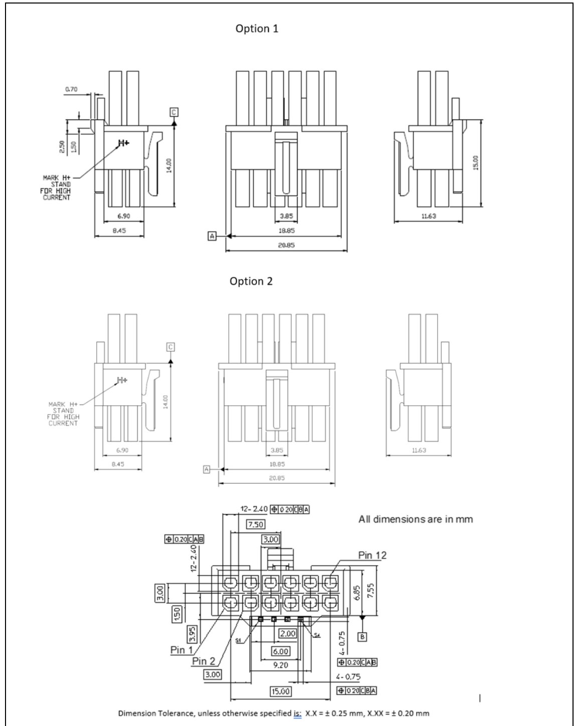
Figure 5-4. 12VHPWR Cable Assembly
