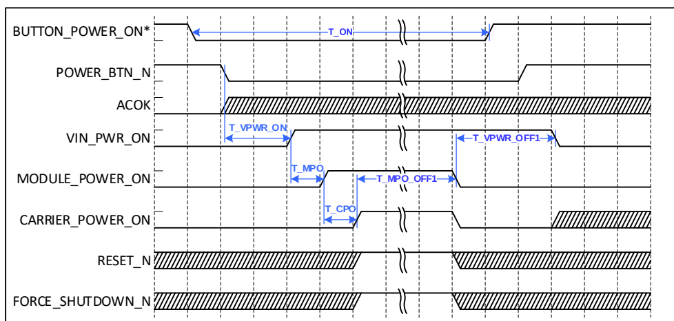
Figure 5-10. Power-On to OFF Power Button Held Low &gt; 10 Seconds
