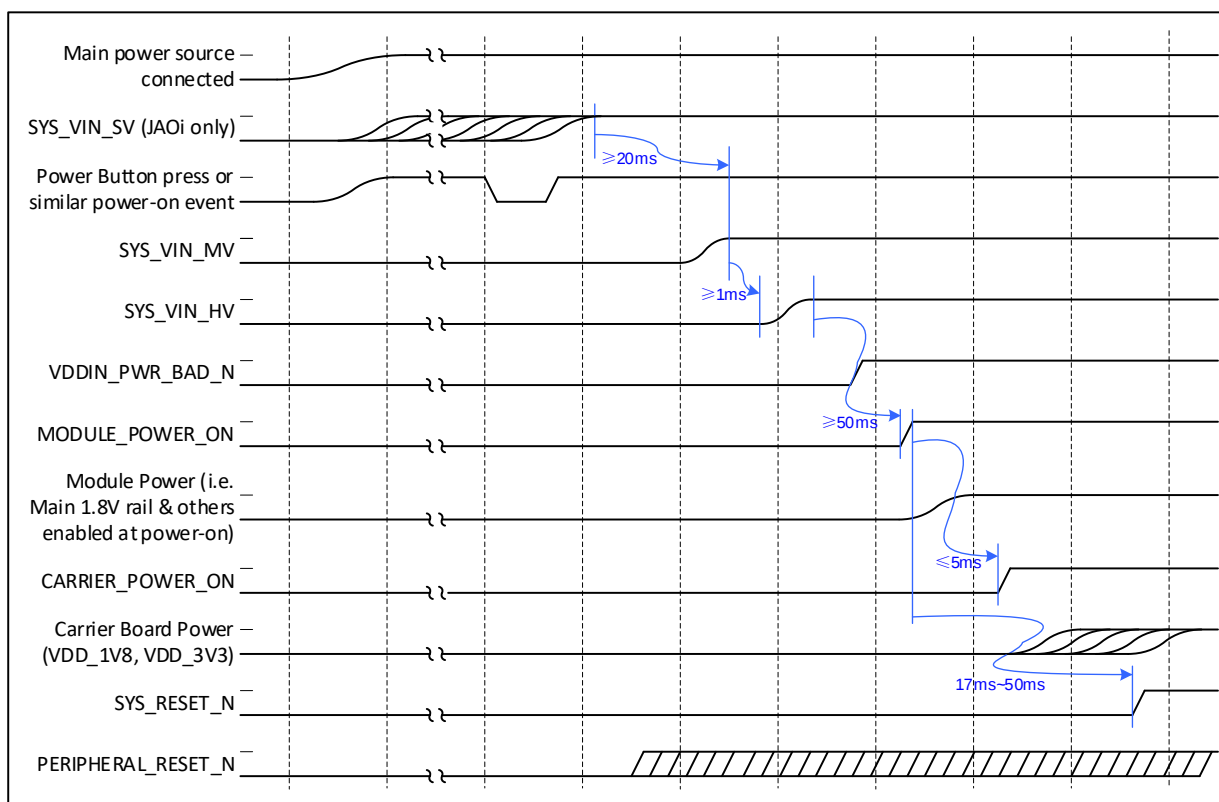
Figure 5-2. Power On Sequence (Power Button Case)
