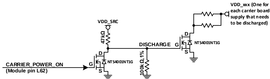
Figure 5-11. Power Discharge
