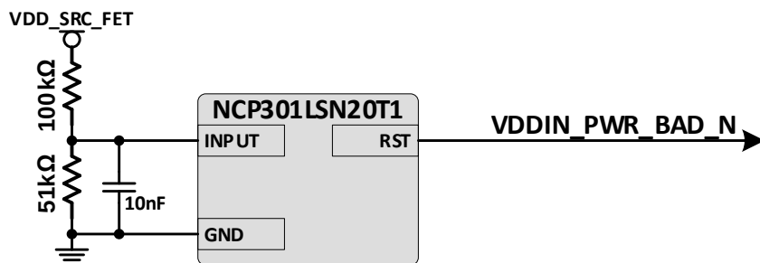
Figure 5-12. VIN Loss Detection Circuit
